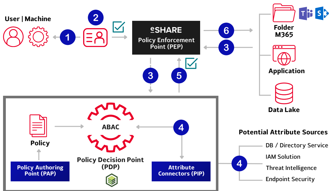
Figure A: ABAC's role in Zero Trust
